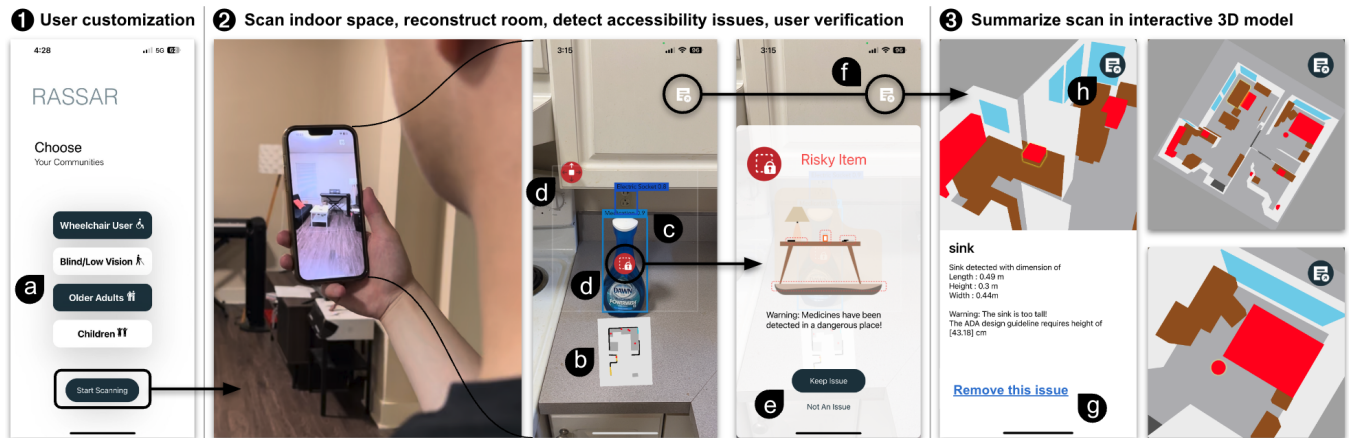
Figure 2: An overview of RASSAR’s user interface and scanning process. The user first (1) selects one or more target communities then (2) manually scans the indoor space to reconstruct the room and detect accessibility and safety issues. Real-time results are shown on a top-down minimap (b) and as bounding boxes and pop-up icons in AR (c and d). The user can click on identified features to view more information, see recommended solutions, and to verify validity. Finally, when the scan is complete (3), we show an interactive 3D model of the room reconstruction with detected issues in red, which can be deleted by clicking (g). Scan results can be saved to JSON for further processing by clicking (h).
